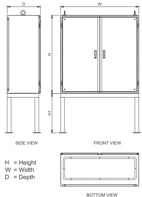
Double Door Control Panel Enclosure
